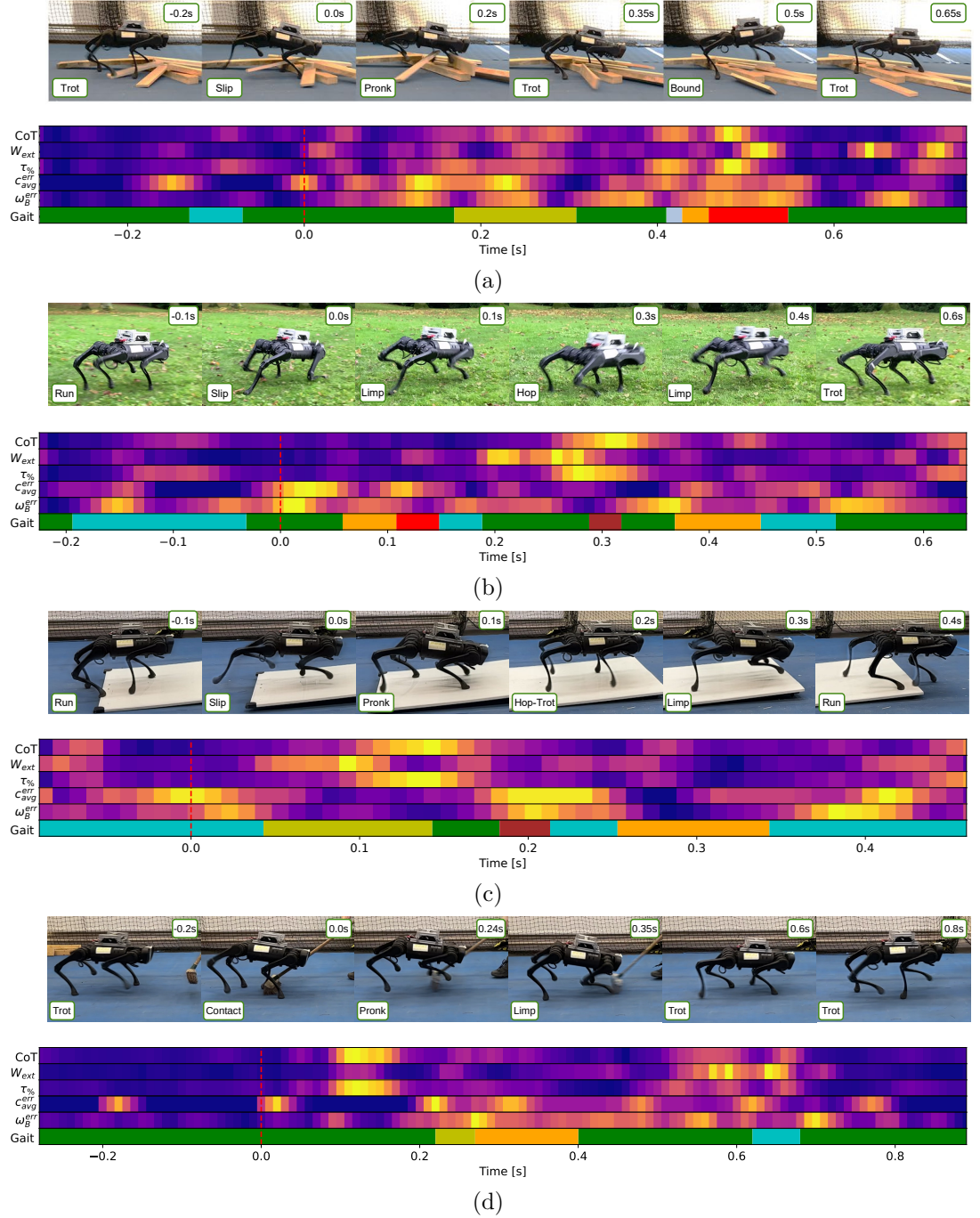
Figure 5.11: The LTA framework is deployed on loose timber, muddy grass, a low-friction board, and subject to perturbations, with maximum velocity magnitudes of 1 m/s, 2 m/s, 1.7 m/s, and 1 m/s respectively, where critical loss of stability is indicated by the red dashed line, the bottom subplot uses the same gait colour code as Fig. 5.6, and the heatmaps show the magnitudes of each metric increasing from purple to yellow.
