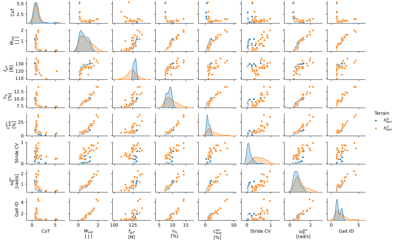
Figure 5.8: Mapping the correlation between metrics and the average gait ID selected across velocities for terrains h^0_{terr} and h^3_{terr} , with the dataset of each terrain consisting of 31 data points averaged over 1000 samples.
