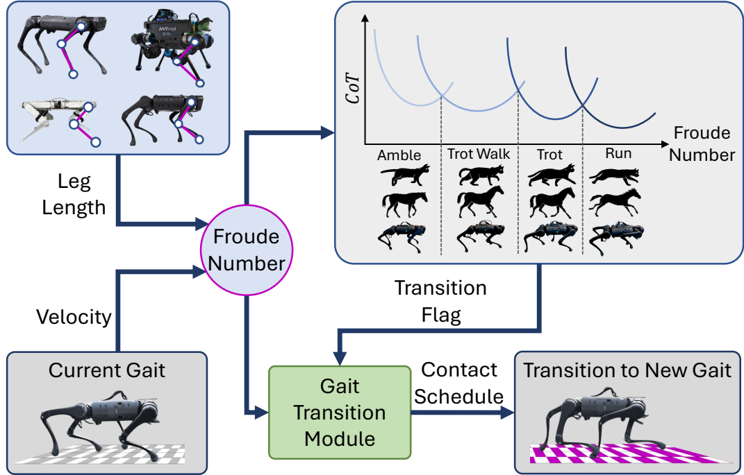
Figure 4.1: An overview of how the Froude number can be leveraged to govern and trigger gait transitions.
