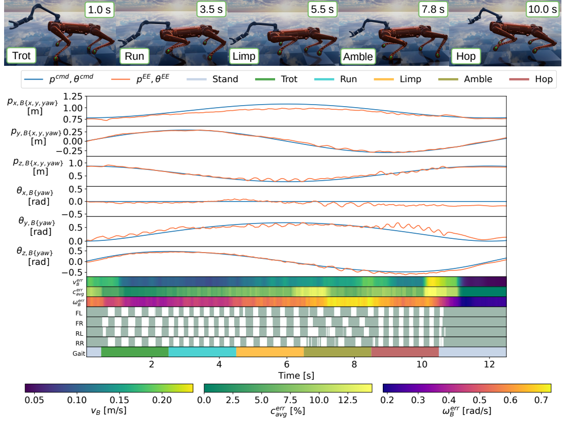
Figure 6.3: Plots of the data collected for the gait switching experiment, with constant base velocity, as depicted in the snapshots at the top of the figure. The top six subplots depict the sinusoidal command \mathbf{p}^{\text{cmd}} , and resultant \boldsymbol{\theta}^{\text{cmd}} , and the realised end-effector tracking of the robot in all 6 DoF. The next three subplots depict the error magnitudes in base velocity command tracking, contact schedule tracking, and base angular velocity. The last plots detail the realised feet contact states and commanded gait.
