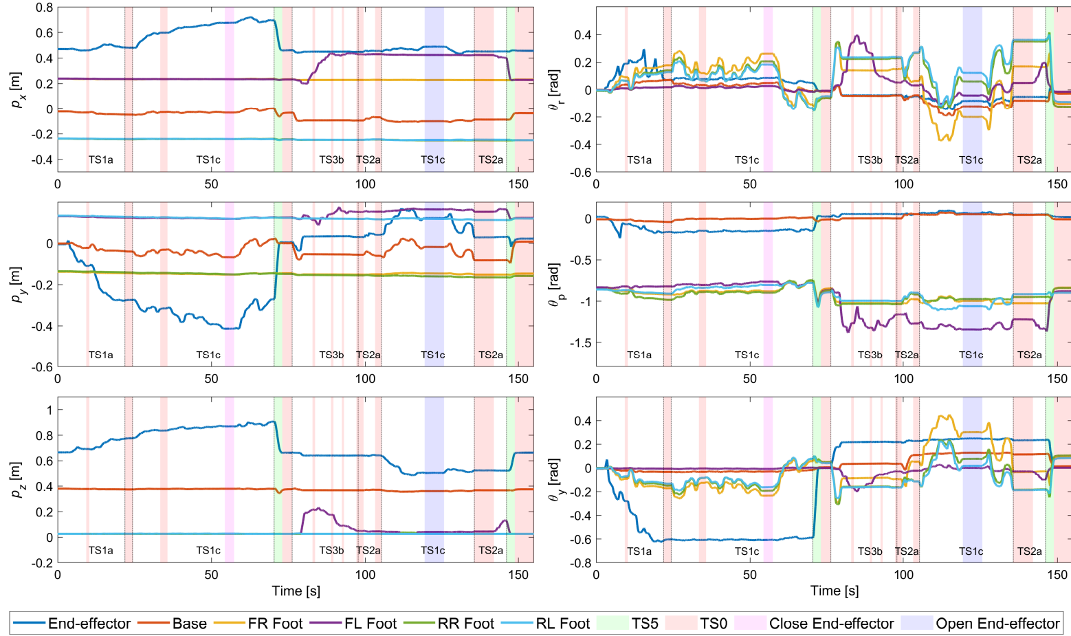
Figure 3.10: The position (left) and orientation (right) WBC and real output of all main frames of the robot during the object disposal experiment.
