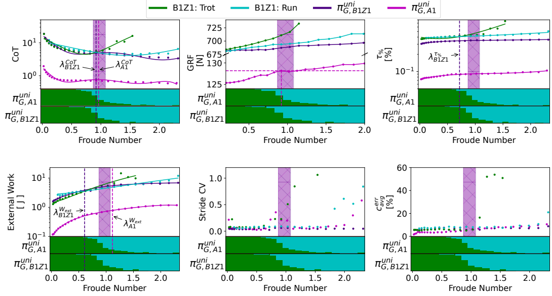
Figure 6.8: Comparing the performance and locomotion characteristics of the retrained \pi_G^{uni} on B1Z1, \pi_{G,B1Z1}^{uni} , with \pi_G^{uni} on A1, \pi_{G,A1}^{uni} , from Chapter 5 to validate successful transfer of animal gait strategies. The A1 data was taken directly from Fig. 5.7. The magenta and purple highlighted regions of the graph represent the gait transition regions (where no single gait occupies more than 75% of the gaits used at a specific Froude number) for \pi_{G,A1}^{uni} and \pi_{G,B1Z1}^{uni} receptively. It should be noted that distinguishing between the transition regions of each robot is rather unclear as they are almost exactly the same.
