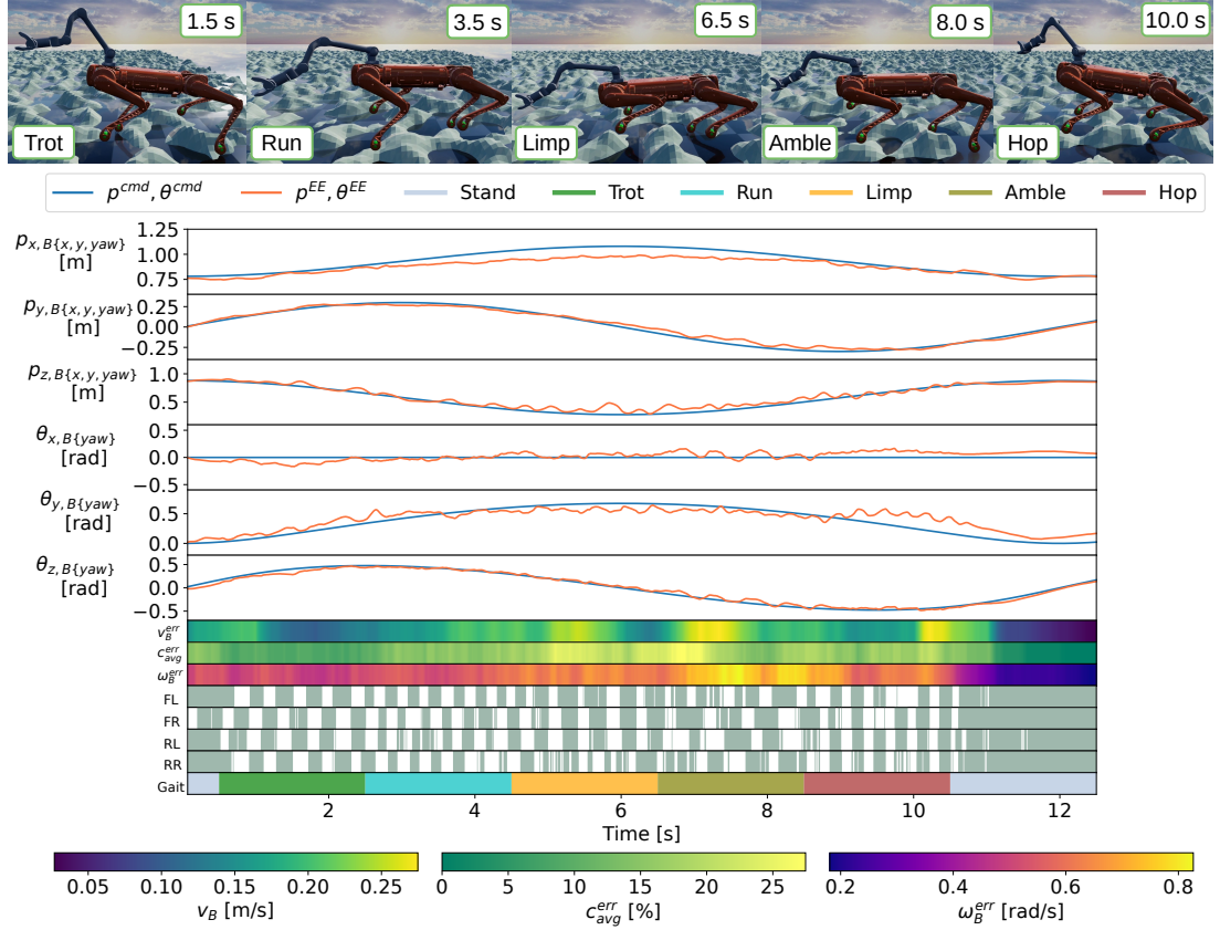
Figure 6.4: Plots depicting the same experiment to that in Fig. 6.3 (using the same graph format) but on rough terrain, featuring a maximum terrain height of 54% of the nominal robot base height. Numerical comparison between rough and flat terrain performance is presented in Table 6.1.
