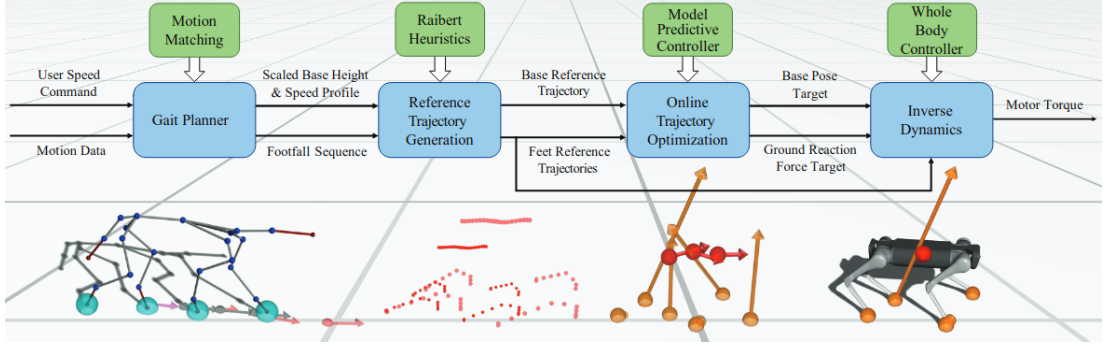
Figure 2.2: The hierarchical optimal control framework developed in [35].
