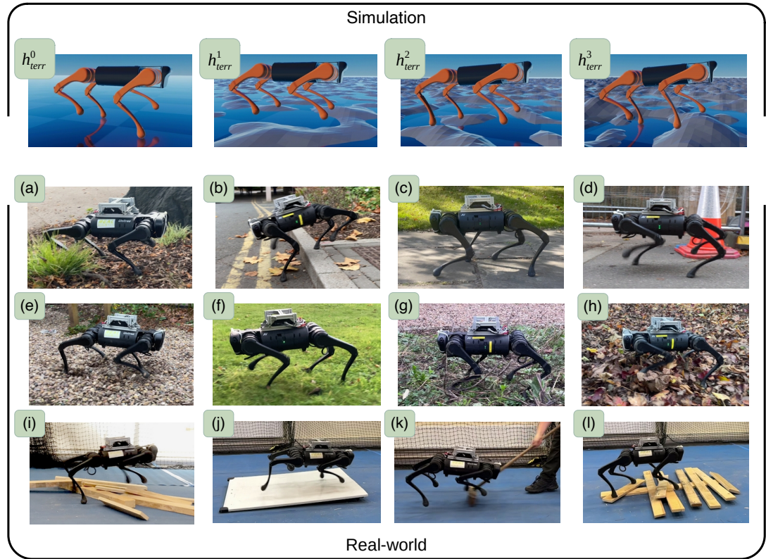
Figure 5.2: Simulated terrains h^0_{terr} through h^3_{terr} are generated with fractal noise with maximum heights of 0 m, 0.06 m, 0.13 m and 0.2 m. The LTA framework has been deployed (a) wood-chip, (b) a large step, (c) concrete slabs with large cracks, (d) tarmac, (e) deep rocks, (f) grassy terrain, (g) overgrown roots, (h) fallen leaves, (i) loose timber, (j) low-friction ramp, (k) flat terrain with perturbations, and (i) balanced timber.
