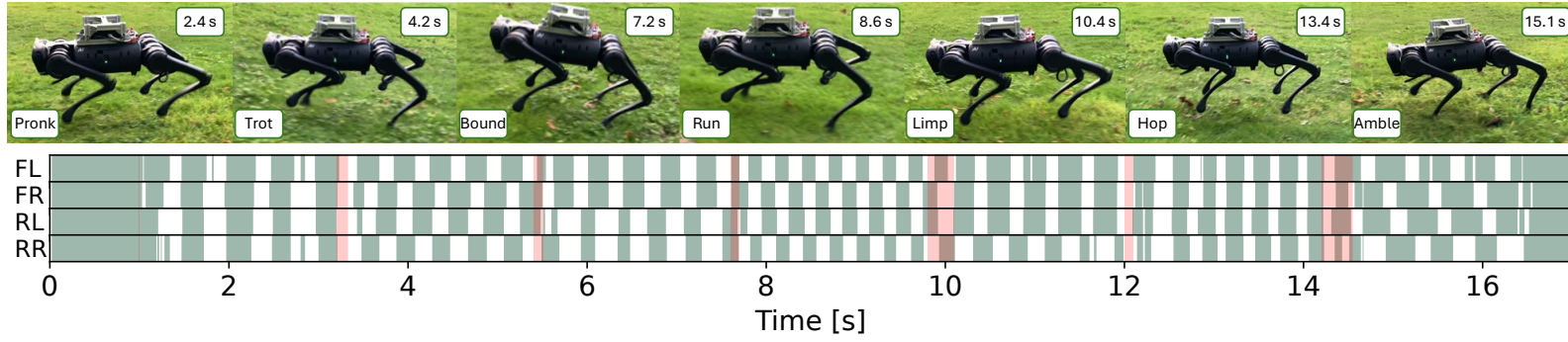
Figure 5.10: The deployment of \pi_L^{\text{bio}} on uneven grassy terrain with manual gait selection to cycle through all gaits with a v_x^{\text{cmd}} of 0.5 m/s where red shaded regions indicate a transition period.
