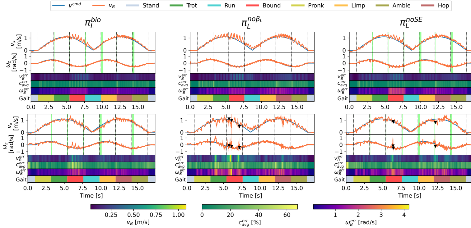
Figure 5.4: Each policy follows a sinusoidal trajectory in x , v_x , and in yaw, \omega_z , while switching gaits every 2 s, which is repeated 5 times over h_{terr}^0 and h_{terr}^3 terrain. Green highlighted areas indicating transition phases, for which the function and formulation are detailed in Section 5.2.2, and black triangles representing points of failure.
