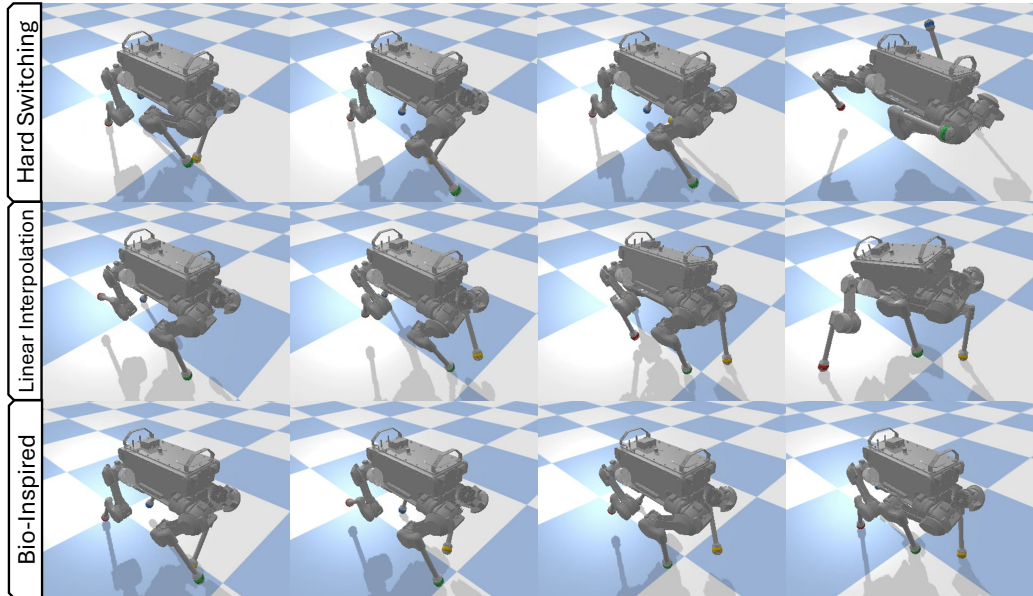
Figure 4.8: A comparison between gait transition methods when transitioning from trot to run at 1.3 \text{ m/s} and 0.4 \text{ m/s}^2 .
