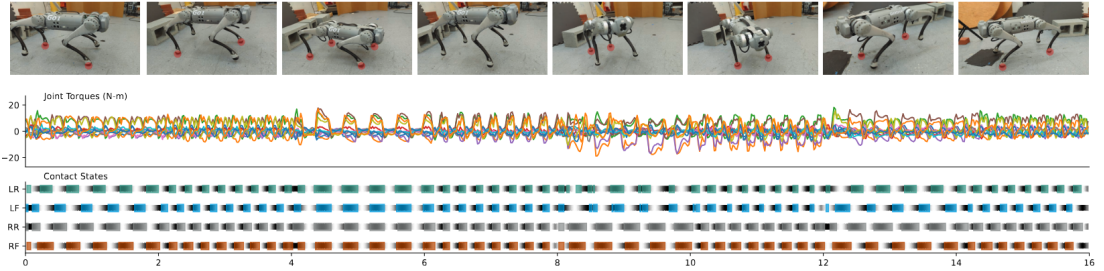
Figure 2.9: Deployment of the DRL policy developed in [104] to realise various gaits, where the top subplot shows the joint torques while the bottom plot shows the contact state of the robot's feet.
