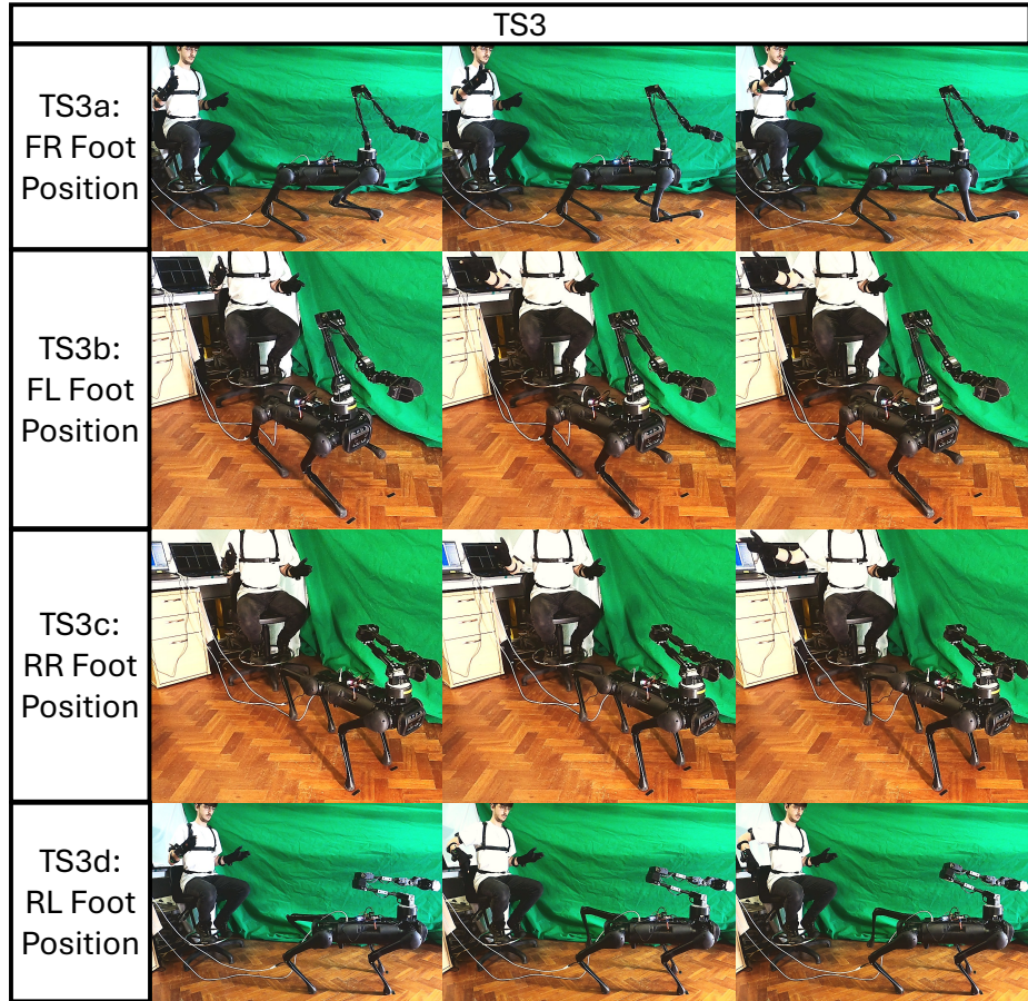
Figure 3.9: Snapshots of using TS3 during the hardware general experiment.
