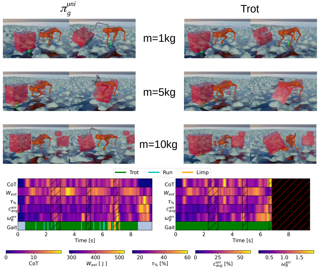
Figure 6.14: This figure details the same experiments and insights to that of Fig. 6.13 but on rough terrain with a maximum terrain height of 54% of the nominal base height. A numerical comparison between rough and low-friction terrain performance is detailed in Table 6.2.
