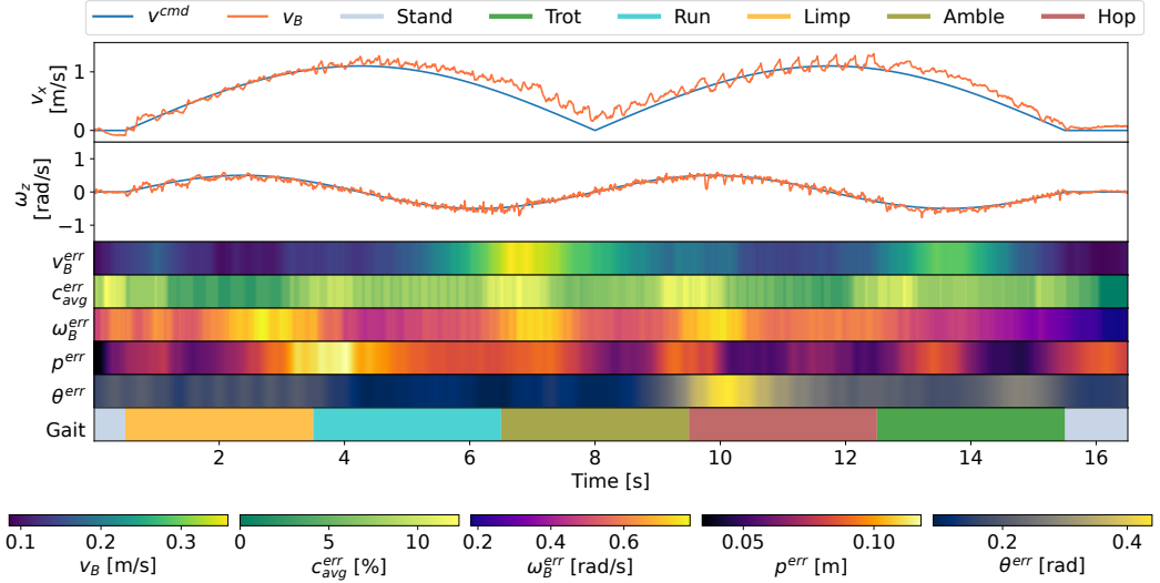
Figure 6.5: The top two plots illustrate the tracking of the robot’s base to the commanded base velocity in x and yaw , following a sinusoidal trajectory. The following six plots, in order, depict the base velocity tracking error, contact schedule tracking error, base angular velocity tracking error, end-effector position tracking error, end-effector orientation tracking error, and the commanded gait.
