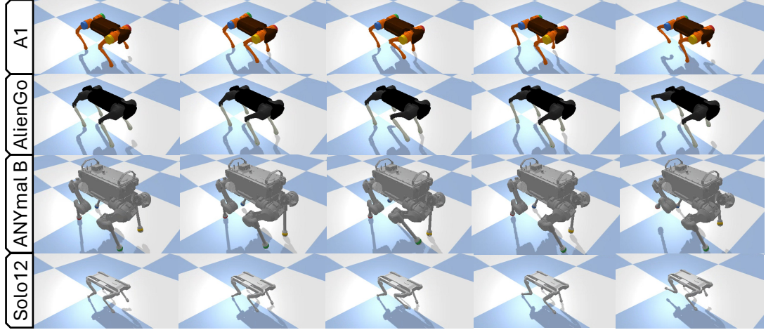
Figure 4.6: The proposed bio-inspired gait transitions has been tested on the A1, AlienGo, ANYmal B and Solo12 Quadrupeds. This figure highlights the transition between amble and walking trot.
