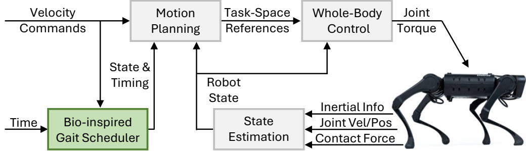
Figure 4.2: The control framework used within this chapter to analyse and validate the proposed BGS.
