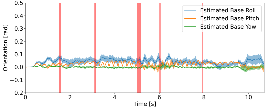
Figure 4.11: Plot of the A1's base roll, pitch, and yaw for all 10 hardware experiments using the developed bio-inspired transition method corresponding with Fig. 4.10.
