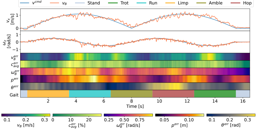
Figure 6.6: Plots depicting the same experiment to that in Fig. 6.5 (using the same graph format) but on rough terrain, featuring a maximum terrain height of 54% of the nominal robot base height. Numerical comparison between rough and flat terrain performance is presented in Table 6.1.
