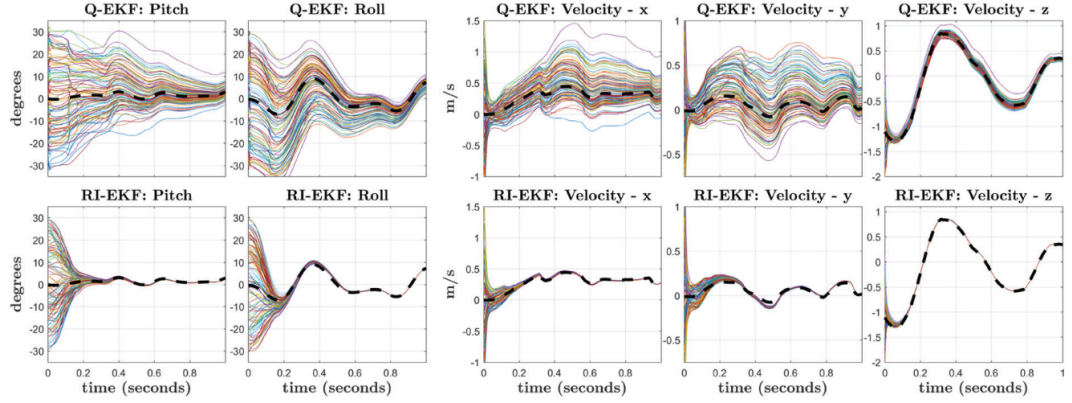
Figure 2.6: A comparison between a quaternion based state estimator and the invariant extended Kalman filter convergence rates developed in [53].
