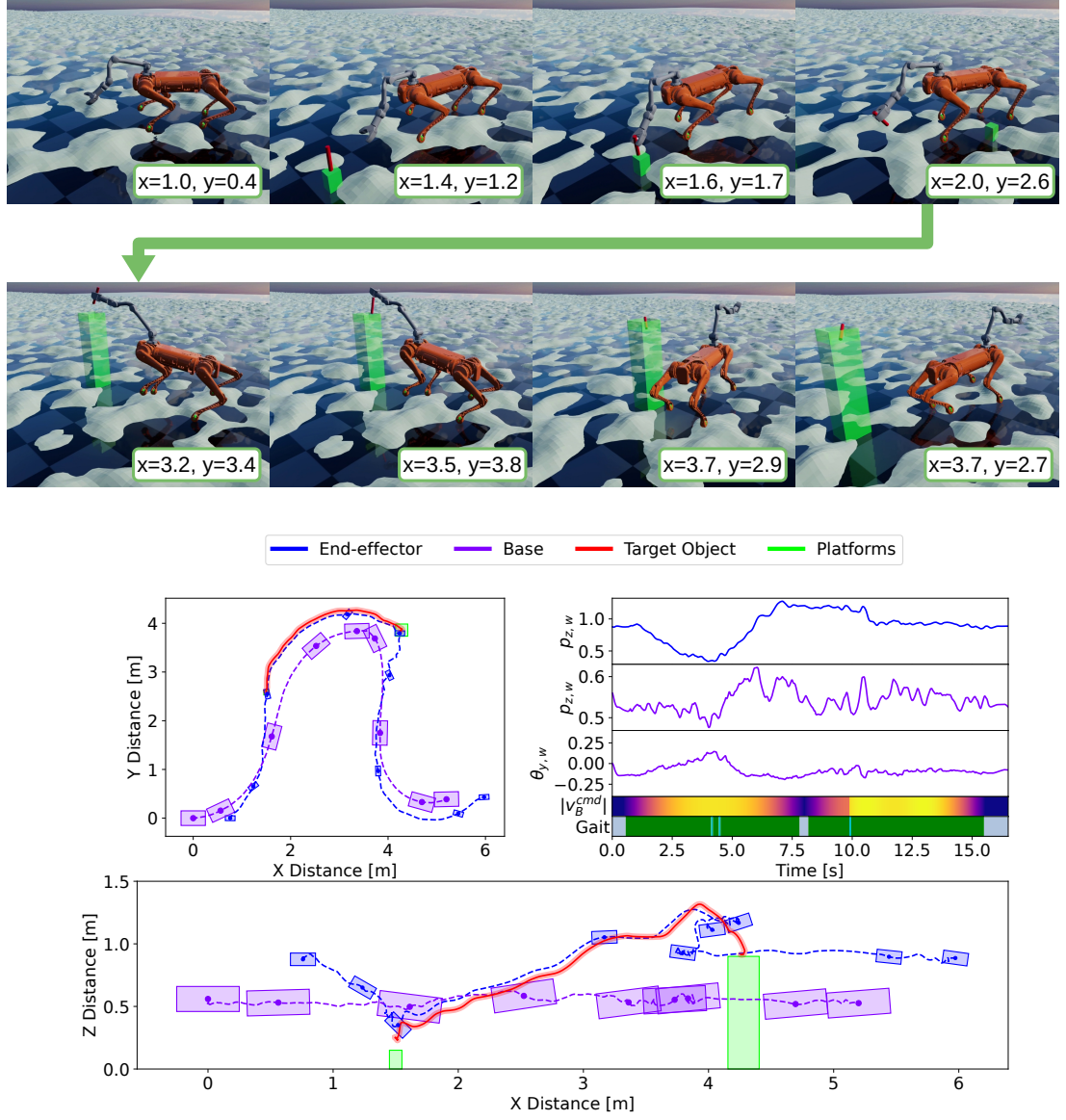
Figure 6.11: This figure details the same experiments and insights to that of Fig. 6.10 but on rough terrain with a maximum terrain height of 35% of the nominal base height.
