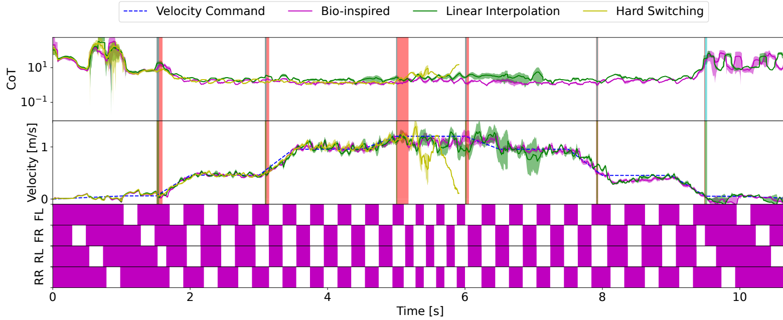
Figure 4.10: Graph showing the CoT, command velocity, estimated velocity, and contact states of the real robot during the experiment (from top to bottom). In the CoT and velocity plots, data from all ten experiments, for each transition method, are presented as average trend lines and variance displaced by the shaded regions. In the bottom four plots, a shaded region shows that a foot is in contact with the ground, while the white spaces show that it is in swing. The bio-inspired gait transition phases are highlighted in red, while the linear interpolation transition phases are in blue.
