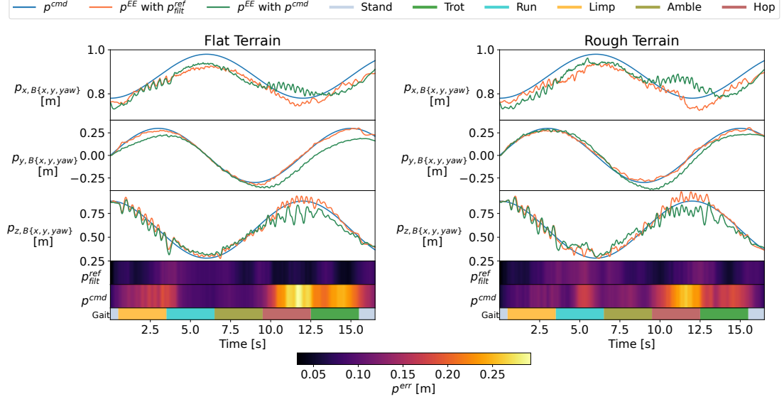
Figure 6.7: A comparison between using the \pi_{LM} action \Delta p^{ref} and just p^{cmd} with no adjustment term as the input reference trajectory for the end-effector Cartesian task within the IK-WBC on flat and rough terrain. The top plots show the end-effector command, when using \Delta p^{ref} , and when using p^{cmd} Cartesian trajectories, while the bottom heatmaps show the normalised (to the maximum and minimum value across all heatmaps) end-effector position error magnitude.
