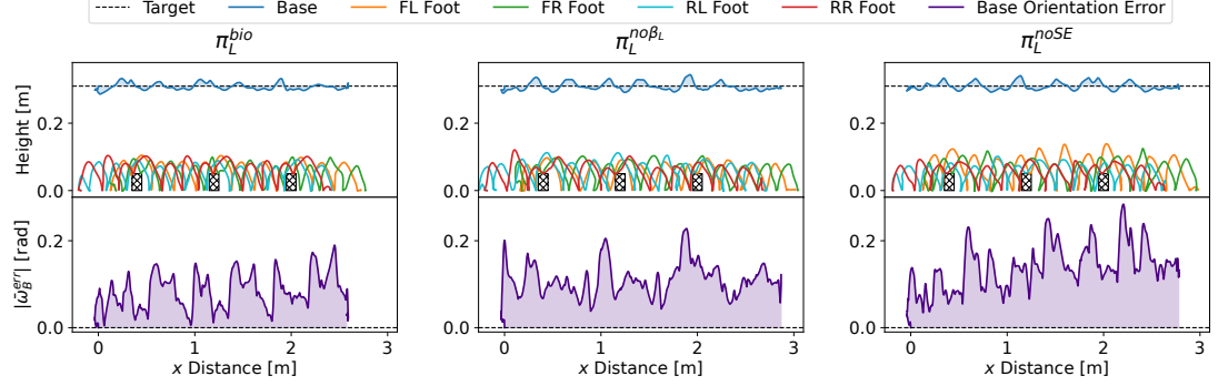
Figure 5.5: Policies follow a command of just v_x = 0.5 m/s while using a constant trot gait while encountering rectangular steps with a height of 0.05 m, where |\bar{\omega}_B^{\text{err}}| is the magnitude of the desired orientation error. FL is front left, FR is front right, RL is rear left, and RR is rear right in reference to the robot’s feet.
