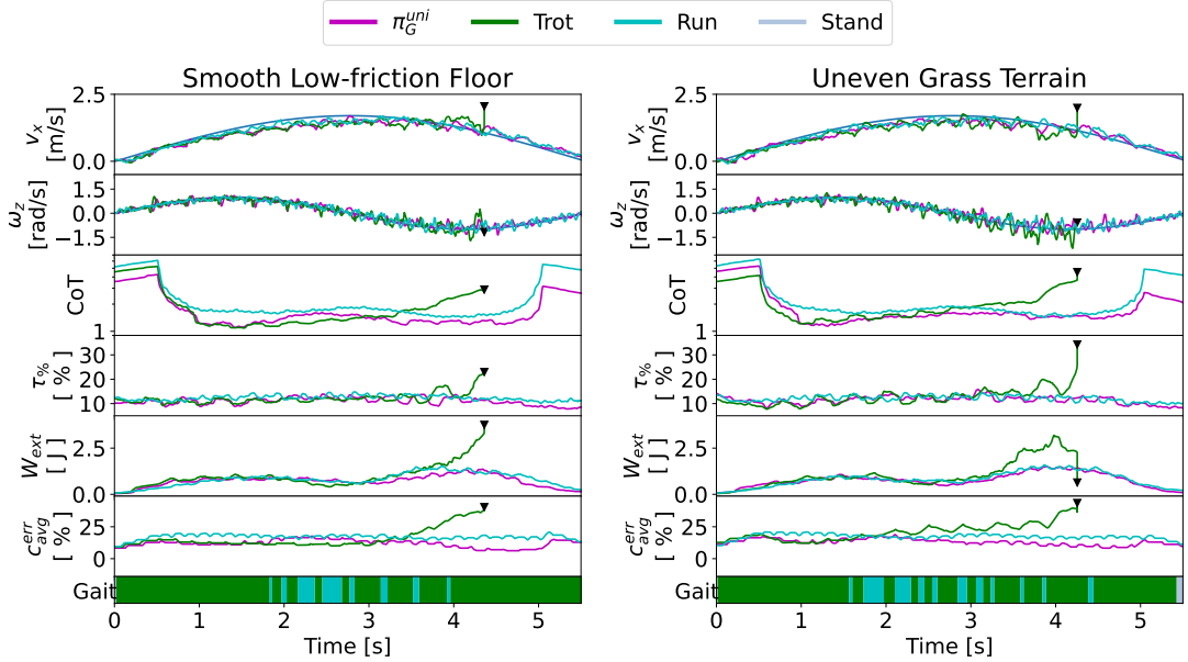
Figure 5.9: Deployment of \pi_L^{\text{bio}} and \pi_G^{\text{uni}} on smooth low-friction floor and uneven grassy terrain, with the black triangles indicating a point of failure.
