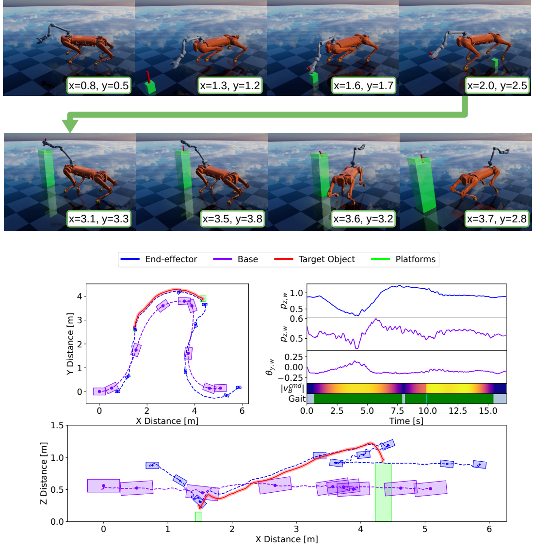
Figure 6.10: The collected data for the pick-and-place task on flat terrain. The top snapshots depict how the robot is able to leverage its redundancy to complete the task. The plots on the left and bottom detail the Cartesian position data of the robot base, end-effector, target object and platforms, while the plot on the right details the timeseries data throughout the experiment to provide an insight into the relationship between the motions of the end-effector and base and the relationship between the base velocity command the selected gait by \pi_{G,B1Z1}^{\text{uni}} . Yaw and pitch orientations are shown for the robot base and end-effector on the x - y and x - z Cartesian plots respectively with 1.8 s intervals as indicated by the boxes drawn at each point.
