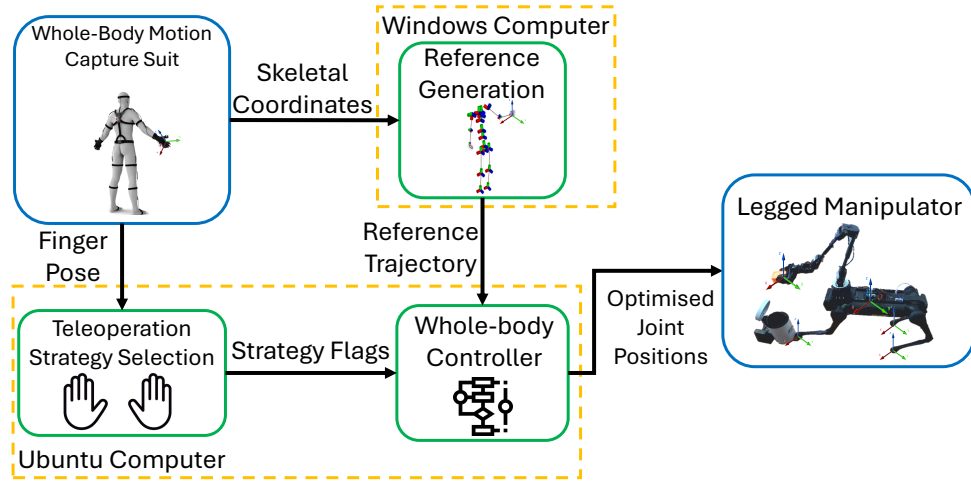
Figure 3.1: System overview of the teleoperation framework to test the IK-WBC.
