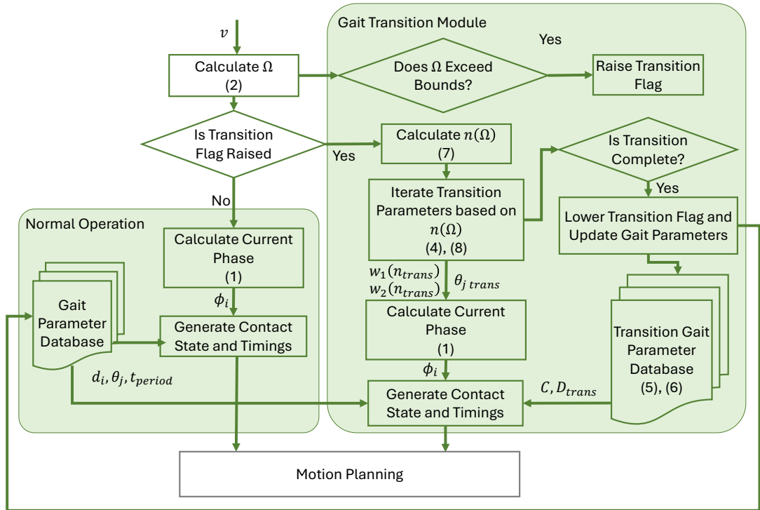
Figure 4.4: Flowchart of the BGS.
