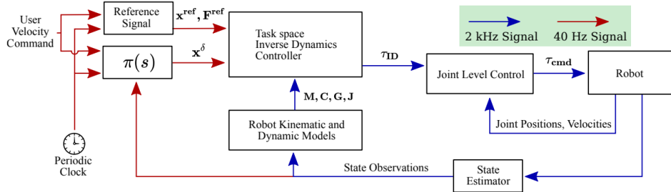
Figure 2.4: An example of a DRL-WBC framework developed in [50].
