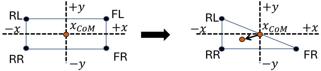
Figure 3.3: Instantaneous translation of the CoM when a foot is no longer in contact with the ground, the orange circles represent the target position and the black circles represent the feet in contact with the ground.
