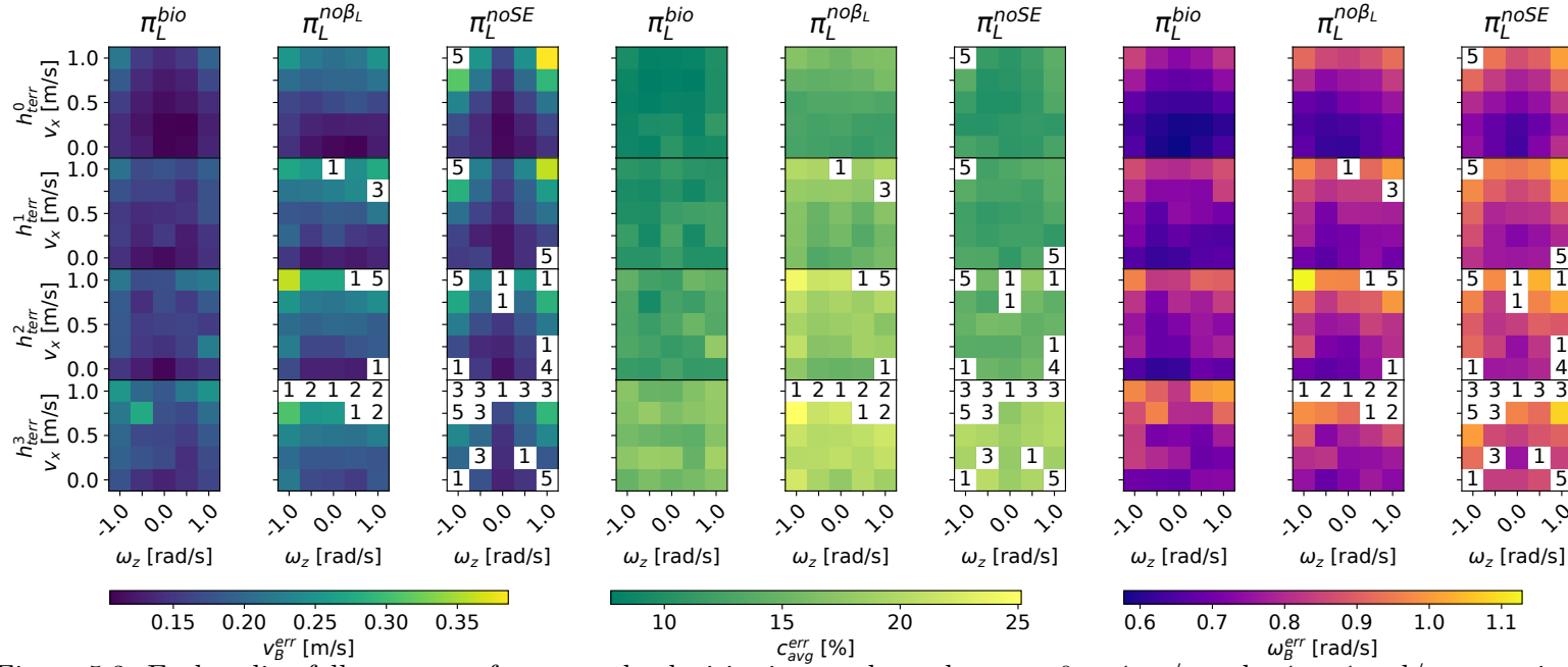
Figure 5.3: Each policy follows a set of command velocities in x and yaw between 0 to 1 m/s and -1 to 1 rad/s respectively. During each velocity pair, the commanded gait is cycled through all gaits, switching every 1 s. This repeated 5 times over flat, h_{terr}^0 , to very rough terrain, h_{terr}^3 (shown in Fig. 5.2) with the average performance being plotted. A number rather than a magnitude indicates the count of experiments that the policy failed.
