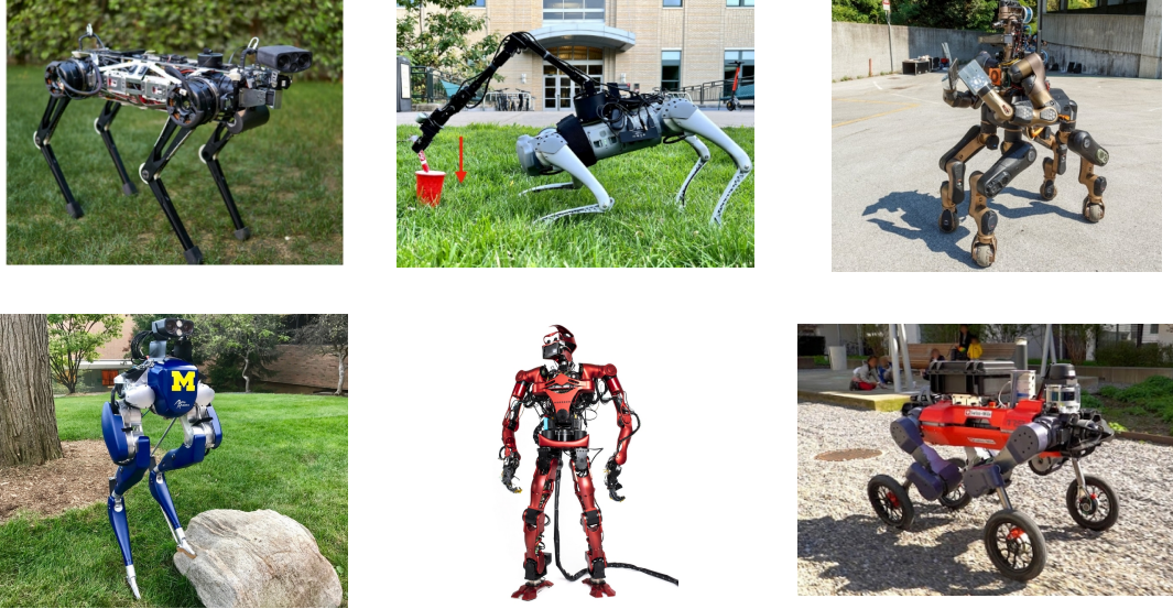
Figure 2.1: Examples of different legged robot morphologies: (from left to right) quadruped [12], quadrupedal legged manipulator [13], wheeled quadrupedal humanoid [14], bipedal [15], humanoid [16], and wheeled quadruped [17]
