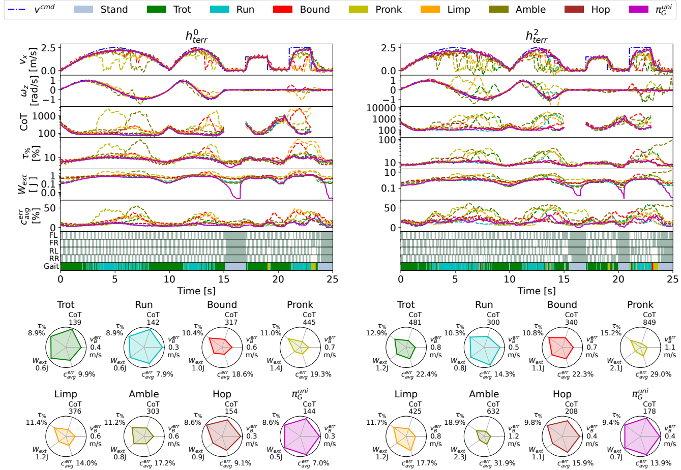
Figure 5.6: For terrains h^0_{terr} and h^2_{terr} , each isolated gait and \pi_G^{uni} are given a velocity command to follow to assess their performance in terms of CoT, \tau\% , W_{ext} , and c^{err}_{avg} ; for each individual gait \pi_L^{bio} just run with the gait statically selected and for \pi_G^{uni} it is coupled with \pi_L^{bio} for autonomous optimal gait selection.
