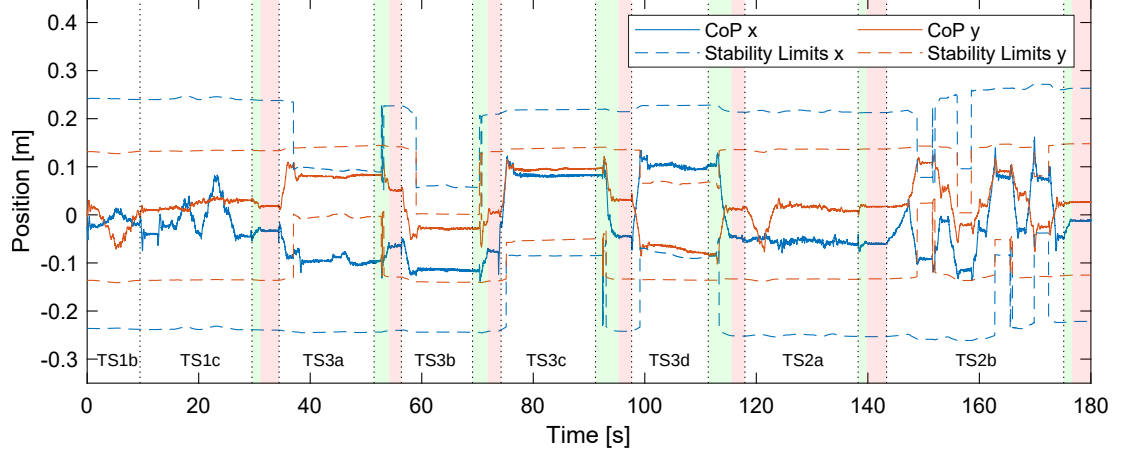
Figure 3.8: x and y components of the robot's CoP during the general demonstration.
