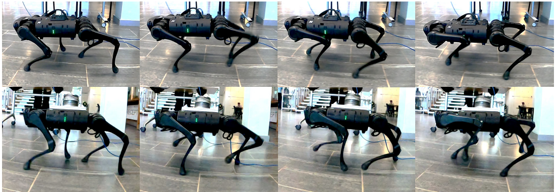
Figure 4.12: Snapshots of the nominal (top) and modified (bottom) A1 during a trot to run transition.
