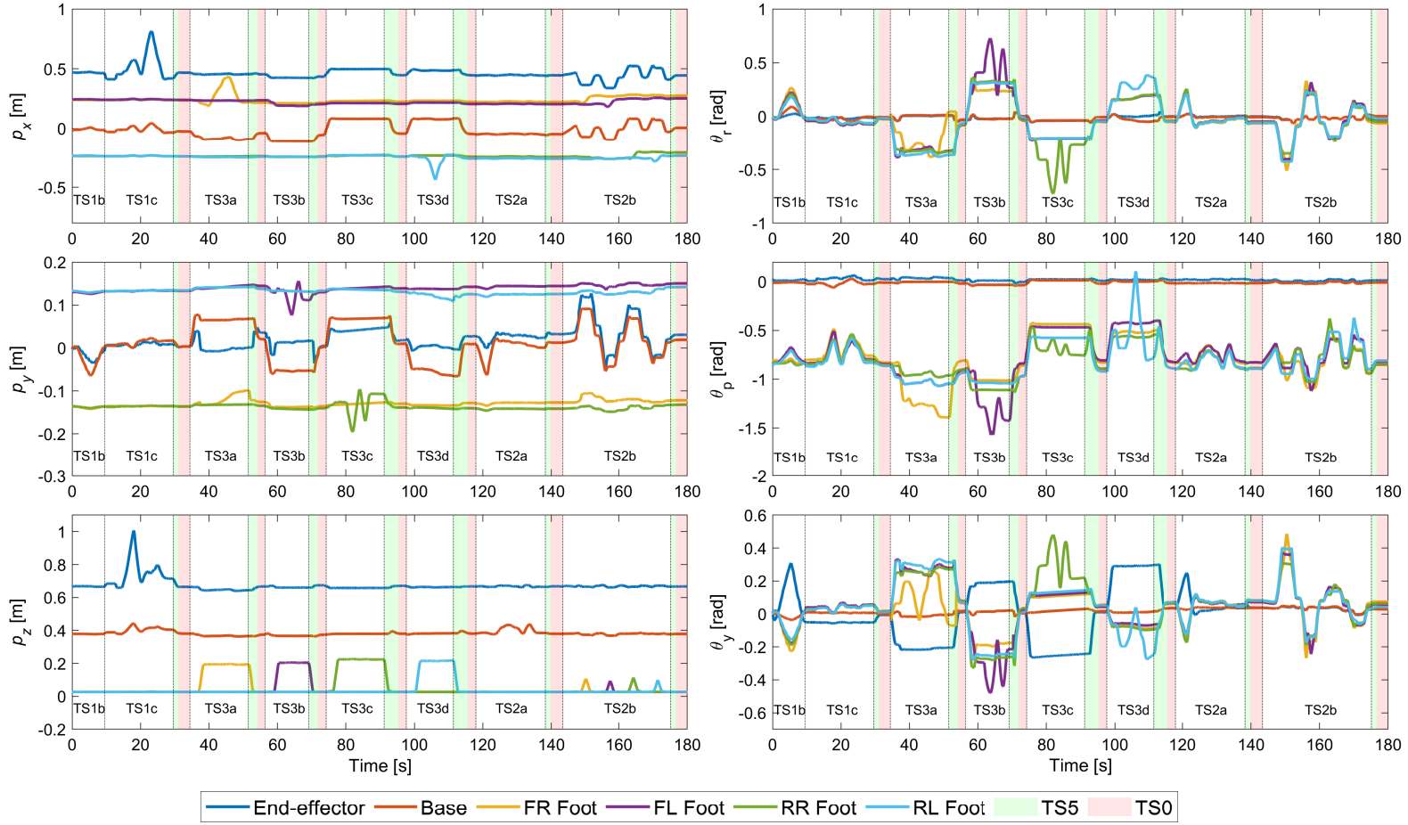
Figure 3.6: The position (left) and orientation (right) WBC and real output of all main frames of the robot during the general demonstration.
