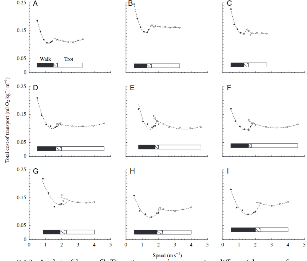
Figure 2.10: A plot of horse CoT against speed across nine different horses, of varying physical statures, to investigate the relationship between CoT preservation and gait transitions [113].
