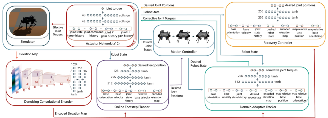
Figure 2.3: The highly complex hybrid control framework developed in [46].
