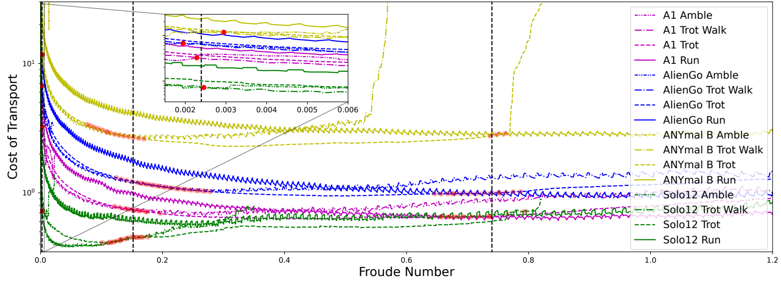
Figure 4.5: To find the optimal points to transition between gaits, a set of gaits are run on the A1, AlienGo, ANYmal B and Solo12 to select and verify the \Omega bounds. This is done through taking a weighted average of points of intersection between subsequent gaits indicated by the red dot markers. Through defining these bounds, as indicated by the black dashed lines, the BGS enables the robot to track the minimal CoT possible with the available gaits as velocity increases.
