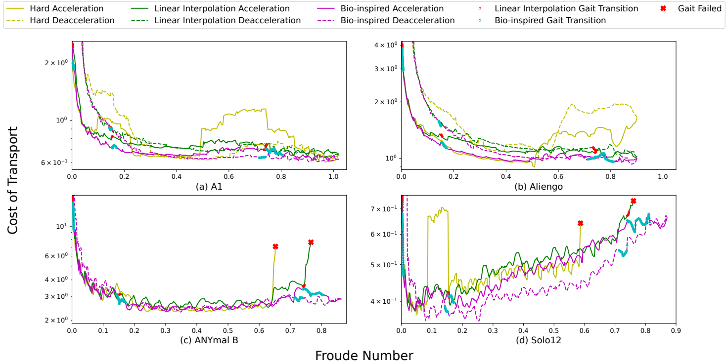
Figure 4.7: Comparing the CoT, the y-axis values, across different gait transition methods with varying \Omega , the x-axis values.
