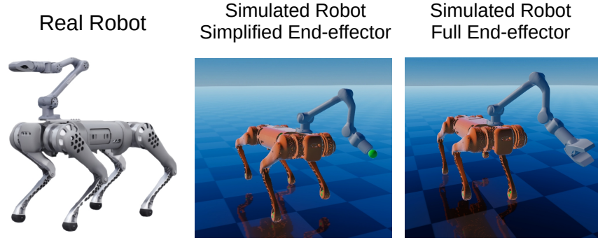
Figure 6.1: Snapshots showing the Unitree Z1 arm mounted on the B1 quadruped, forming the legged manipulator to be used in this Chapter. During training the end-effector was simplified, indicated by the green sphere in the middle snapshot, to reduce training time.
