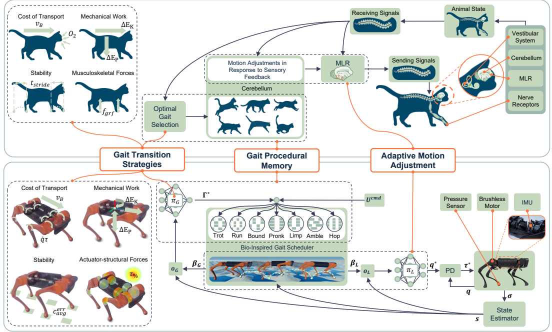
Figure 5.1: The LTA Framework. From taking an abstracted view of animal locomotion to determine the attributes of proficient locomotion, animal gait transition strategies are instilled within the gait selection policy, \pi_G , gait procedural memory is embedded within the bio-inspired gait scheduler, and adaptive motion adjustments are realised by the locomotion policy, \pi_L . \pi_G has been trained to minimise the animal gait transition metrics applied to the quadruped robot based on the current robot state, \mathbf{s} , and relevant bio-inspired gait scheduler output, \beta_G , to select the optimal gait, \Gamma^* . The bio-inspired gait scheduler then generates the gait references informed by \mathbf{s} from encoded high-level gait parameters. The gait references, \beta_L , are then passed to \pi_L to inform of any adjustments to the nominal gait motions. The control framework is constant between training and deployment to improve sim-to-real transfer. Regarding acronyms, MLR is, mesencephalic locomotor region, PD is proportional derivative controller, and IMU is inertial measurement unit.
