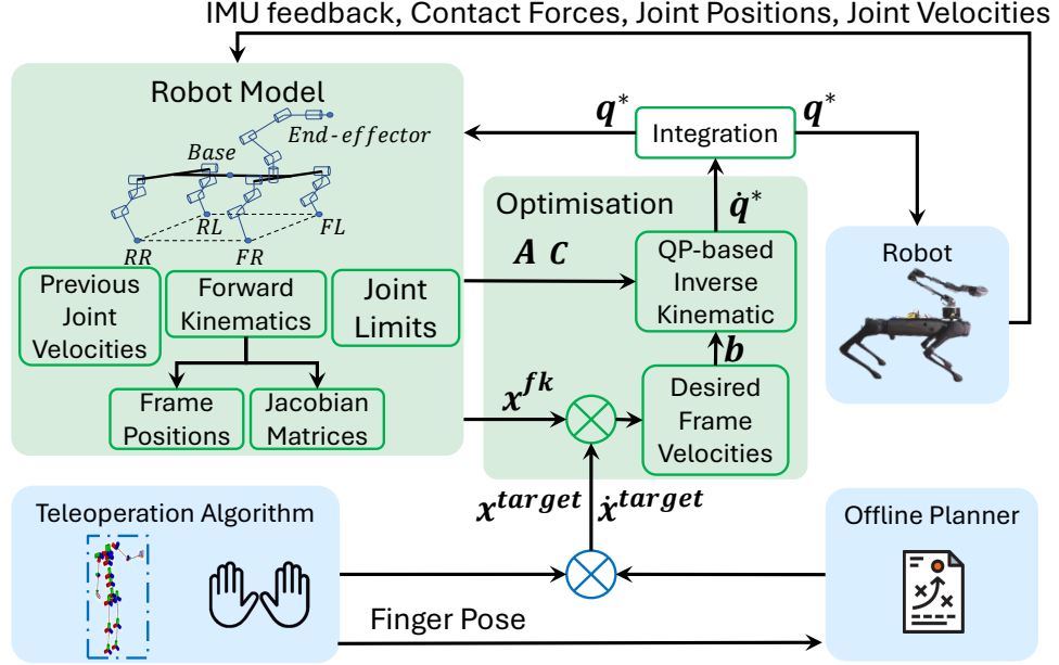
Figure 3.2: Block diagram of the IK-WBC, built around the QP problem.
