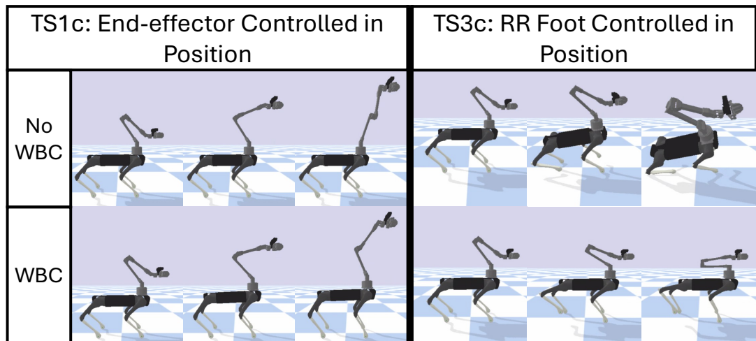
Figure 3.5: Comparing the performance with and without the WBC enabled.
