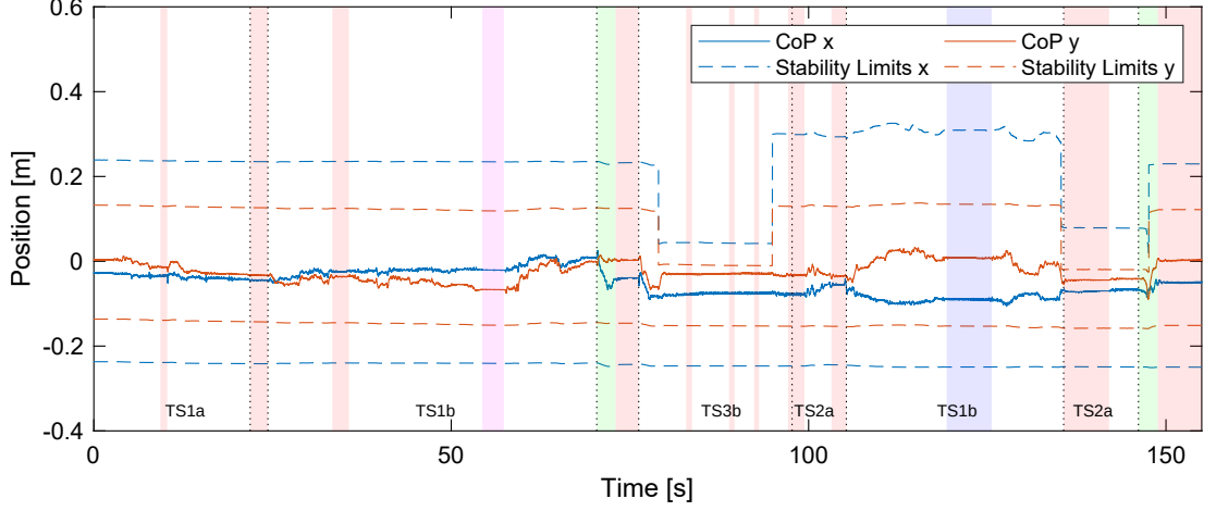
Figure 3.11: The x and y components of the robot’s CoP during the object disposal experiment.
